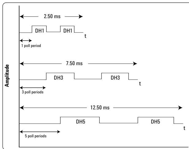
Figure 28. Timing diagram for test set for each packet type. Use with External Frame Sync not selected. Use with External Frame Sync is selected, the DH1 impairment set consists of four packets.
