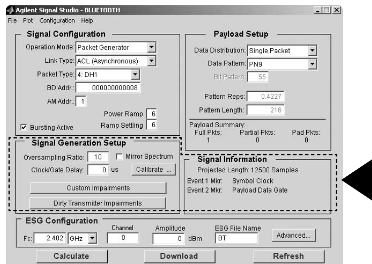
Figure 17. Signal Generation Setup and Signal Information menus.
