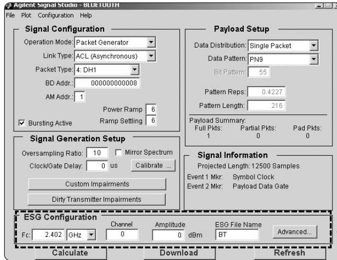
Figure 34. ESG Configuration menu.
