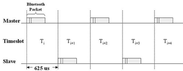
Figure 1. Bluetooth time-division duplex transmission scheme.
