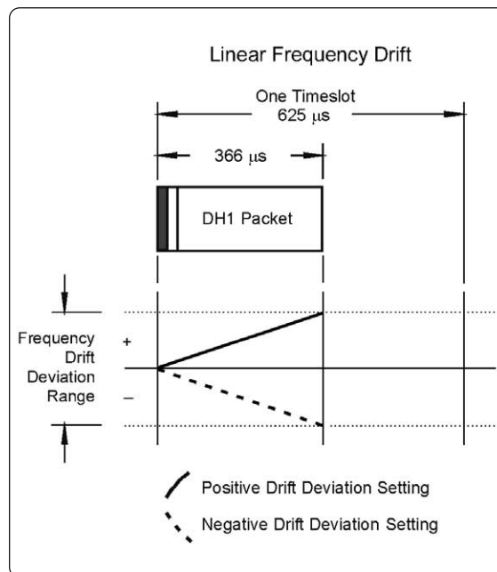
Figure 33. Linear frequency drift impairment
