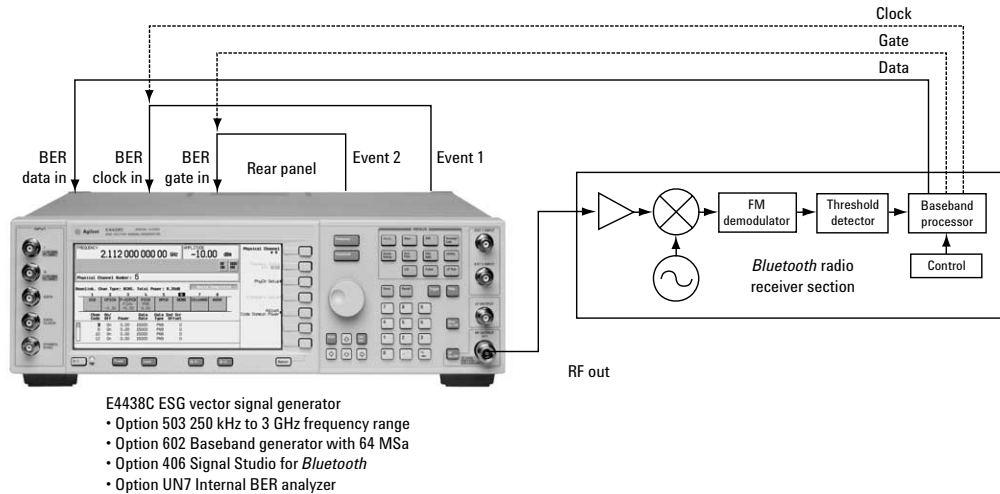
Figure 40. BER test setup for a Bluetooth device in “continuous receive” operating mode. Note: Dashed lines indicate alternate configurations.
