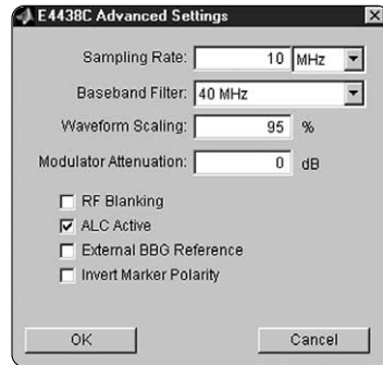
Figure 35. E4438C Advanced Settings menu.
