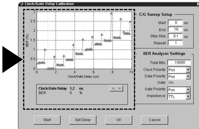
Figure 46. BER vs. Clock/Gate Delay calibration results.
