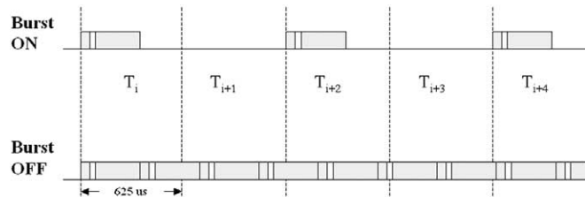
Figure 16. Bursted and non-bursted single slot packet transmission.
