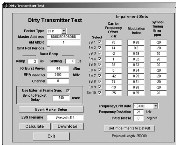
Figure 25. Dirty Transmitter Test menu
